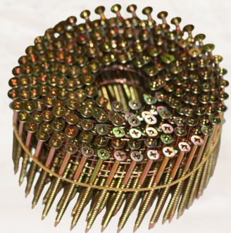
15° Wire Coil
